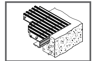
2-1/2" grating: PN# 1618005 Install 2-1/2" side vertical
