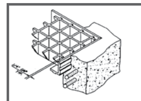
2" grating: PN# 1617900 Install 2" side vertical
