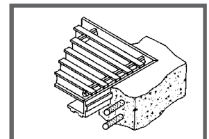
1-1/2" grating: PN# 1617900 Install 1-1/2" side vertical
