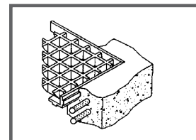
1" grating: PN# 1617910 Install 1" side vertical
